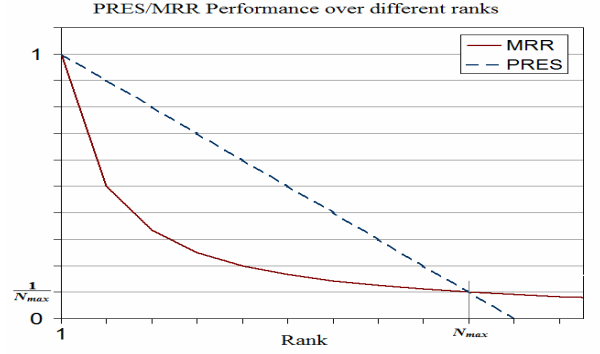
Figure 4(b). PRES vs MRR for different rank when n=1
