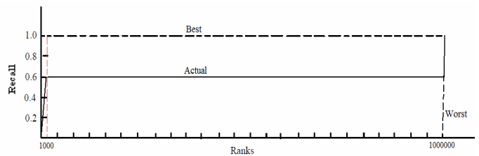
Figure 2. Illustration of how R_{norm} curve behaves with large document collections
