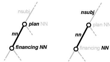
Figure 1: Lexicalised and unlexicalised features sets
