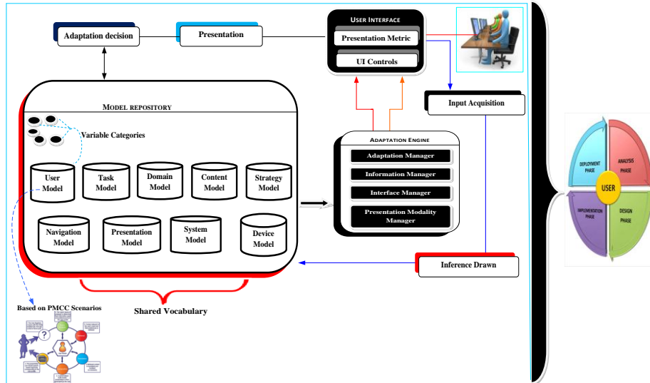
Figure 1: Architectural design for Frameworks of UCEAS: Module 1
