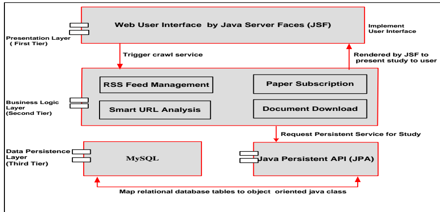
Figure 2: Architectural design for Frameworks' Module 2
