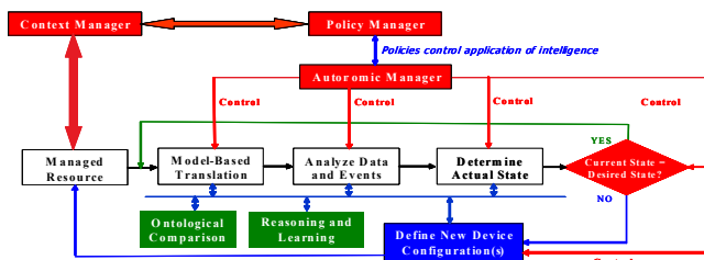
Figure 3. FOCALe Conceptual Autonomic Architecture
