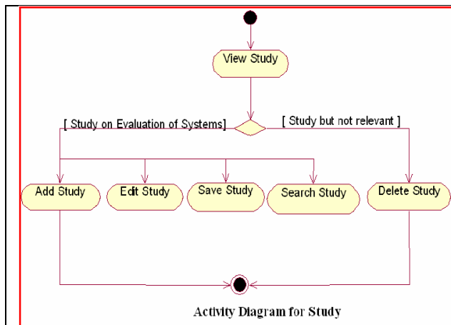
Figure 4: Activity Diagram
