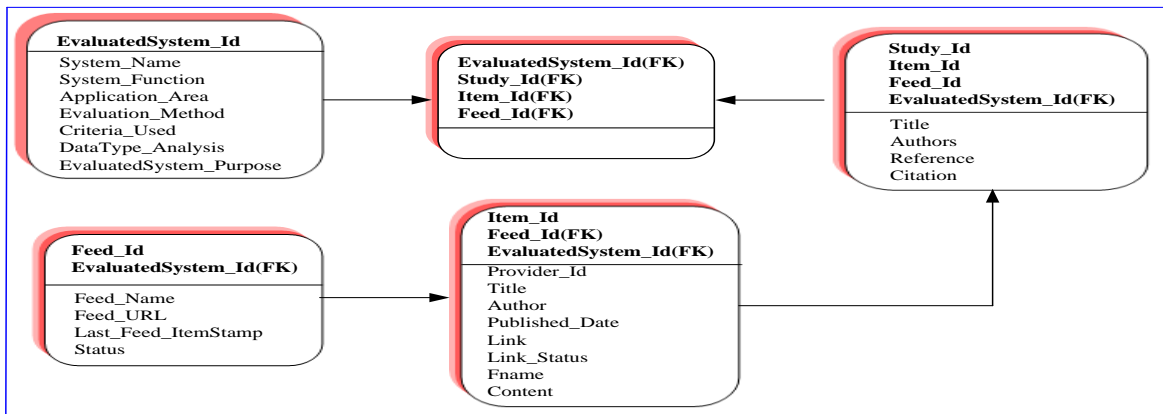
Figure 3: OSSES Database Design
