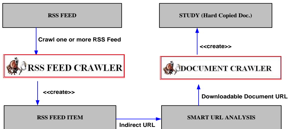
Figure 2 Crawling Process
