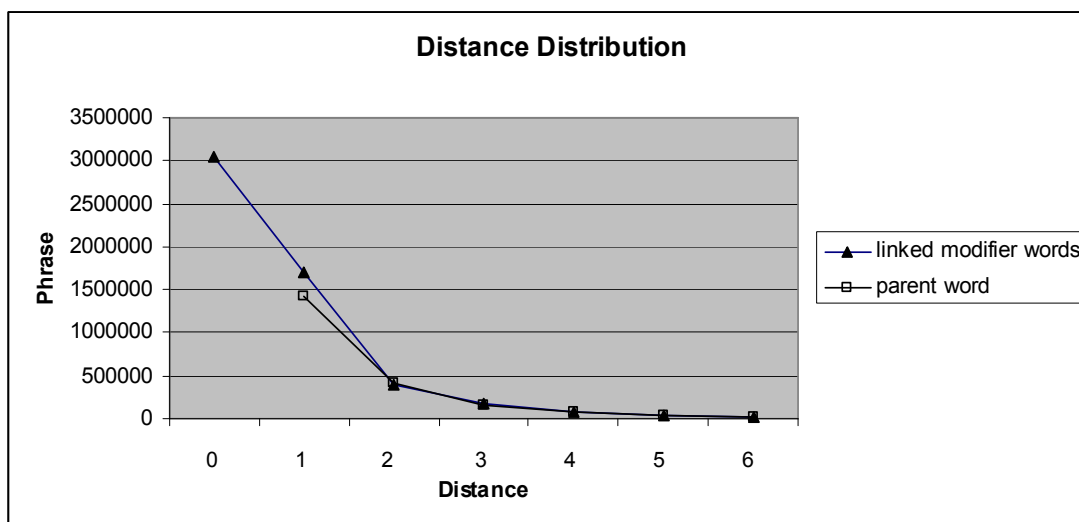
Figure 1: Distances found between phrase boundaries with linked modifier words and parent word.
